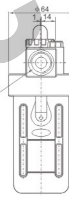
BR2000: G1/4" BR3000: G3/8" BR4000: G1/2"
